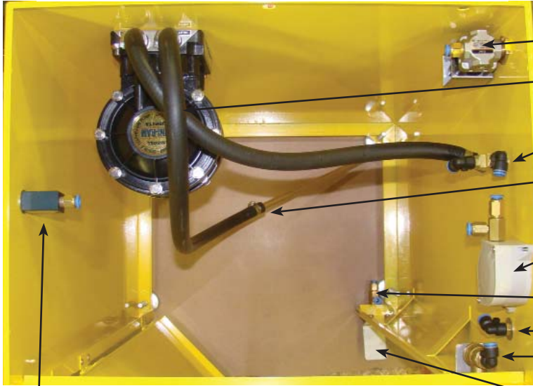
TOP VIEW OF LOWER CABINET, LOOKING DOWN
